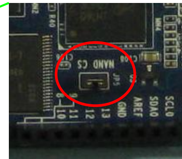
NAND_CS jumper
